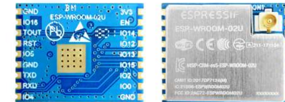
Figure 3-4. ESP-WROOM-02U Module
