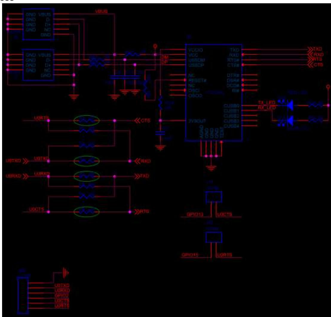
Figure 2-2. ESP-LAUNCHER Interface
