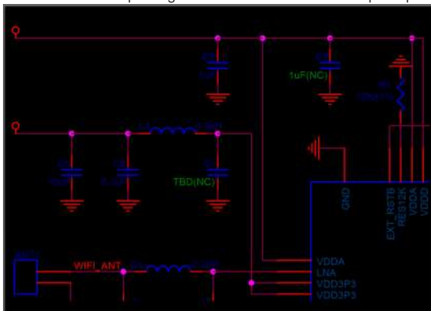
Figure 1-5. ESP8266EX AVDD
