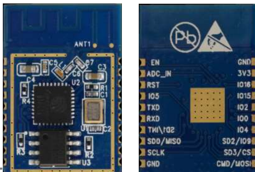
Figure 3-1. ESP-WROOM-S2 Module
